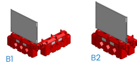
Nexus Barrier + Hoarding Panel Buttressed
