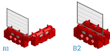
Nexus Barrier + Mesh Fence Panel Buttressed
