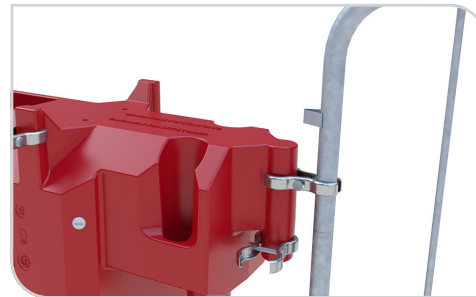
Nexus Barrier connected with 2.3m Pedestrian Barriers
