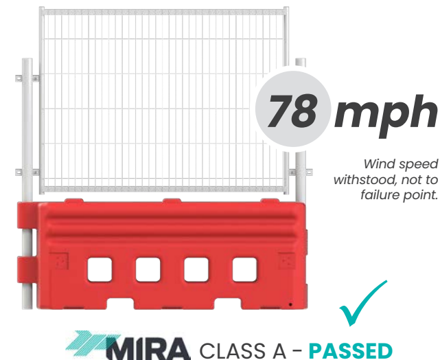
2 RB22 Barrier + Mesh Fence Panel
