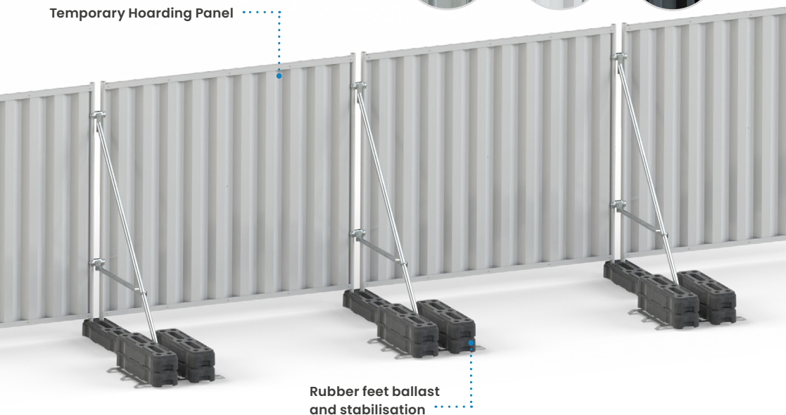
Temporary Hoarding Panel
