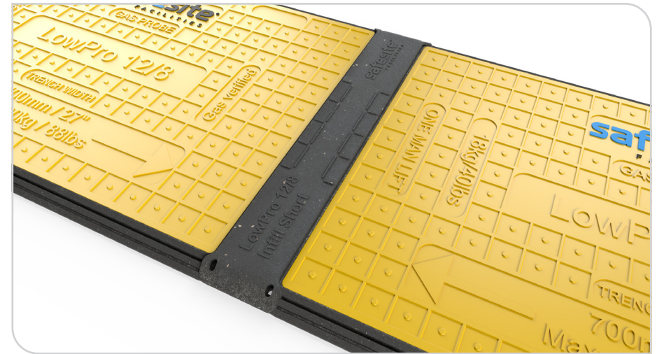
Short Infill strips connected with LowPro 12x8 Trench Cover
